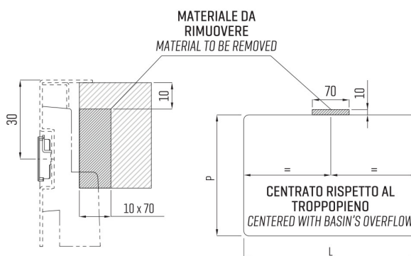
TROPPOPIENO OVERFLOW HOUSING DETAIL
