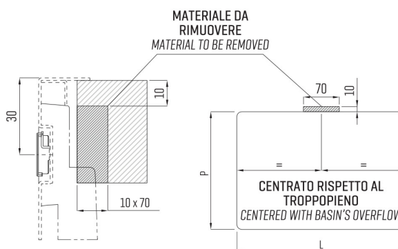
TROPPOPIENO OVERFLOW HOUSING DETAIL
